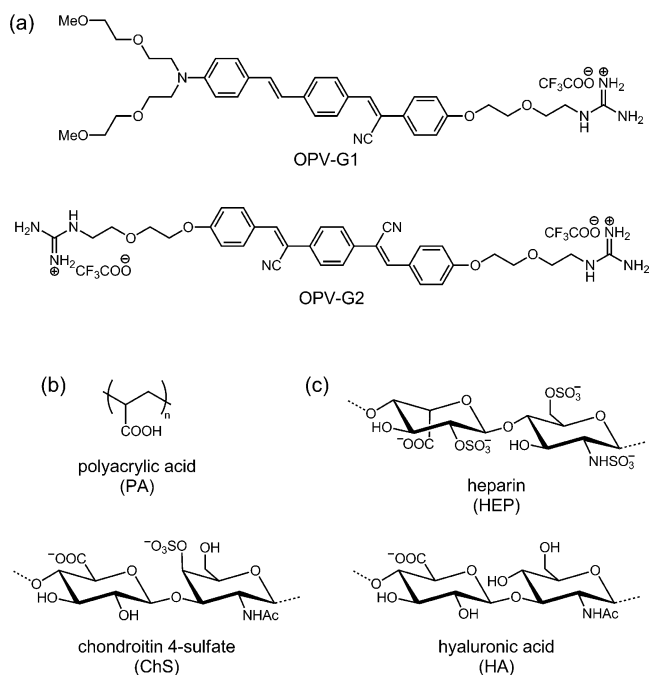
Figure 1. Chemical structures of a) assembly-based fluorescent chemosensors: OPV-G1 and OPV-G2, b) polyacrylic acid (PA), and c) representative glycosaminoglycans: heparin (HEP), chondroitin 4-sulfate (ChS), and hyaluronic acid (HA).
