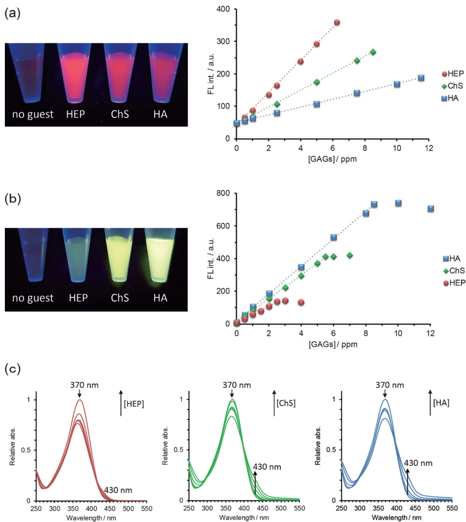
Figure 4. a) Photograph of OPV-G1 in the absence and presence of HEP (6.25 ppm), ChS (8.50 ppm), and HA (11.5 ppm), and changes in the fluorescence intensity of OPV-G1 upon increasing concentrations of HEP (red), ChS (green), and HA (blue). Conditions: [OPV-G1] = 30 \mu M, [HEPES] = 10 mM (pH 7.4), 25 ^{\circ} C, \lambda_{\text{ex}} = 400 nm. b) Photograph of OPV-G2 in the absence and presence of HEP (2.5 ppm), ChS (5.5 ppm), and HA (8.5 ppm), and changes in the fluorescence intensity of OPV-G2 upon increasing concentrations of HEP (red), ChS (green), and HA (blue). c) UV/Vis titration of OPV-G2 upon increasing concentrations of HEP (red), ChS (green), and HA (blue) in HEPES buffered water. Conditions: [OPV-G2] = 10 \mu M, [HEPES] = 10 mM (pH 7.4), 25 ^{\circ} C, \lambda_{\text{ex}} = 388 nm.
