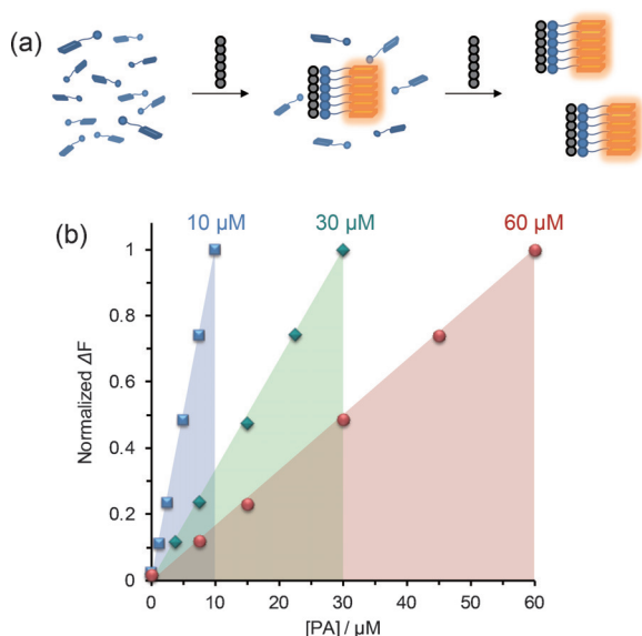
Figure 3. a) Schematic illustration of PA sensing that exhibits apparent 1:1 linear relationship. b) Dependence of OPV-G1 concentration (blue: 10 \mu\text{M} , green: 30 \mu\text{M} , red: 60 \mu\text{M} ) on the detection range toward PA (0–1.0 equivalent).
