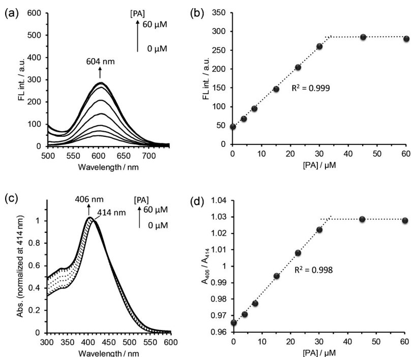
Figure 2. a) Fluorescence titration ( \lambda_{\text{ex}} = 400 \text{ nm} ) of OPV-G1 upon increasing concentration of PA (0–60 \mu\text{M} ) in HEPES buffered water. b) Plot of the changes in the fluorescence intensity at 604 nm. c) UV/Vis titration of OPV-G1 upon increasing concentration of PA (0–60 \mu\text{M} ) in HEPES buffered water. d) Ratiometric plot of A_{406}/A_{414} . Conditions: [OPV-G1] = 30 \mu\text{M} , [HEPES] = 10 mM (pH 7.4), 25 ^{\circ}\text{C} .
